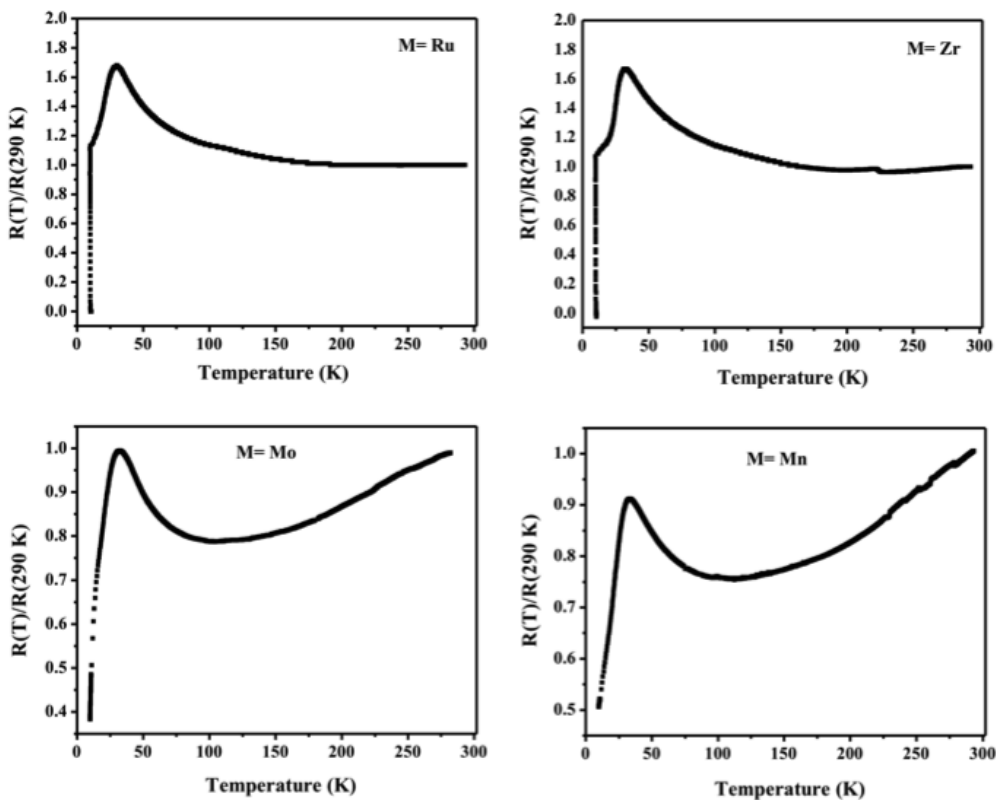
Fig. 4. Normalized resistance as a function of temperature of the \text{Ru}_{0.9}\text{M}_{0.1}\text{Sr}_2\text{GdCu}_2\text{O}_8 system, with M = \text{Ru} , Zr, and Mn.
