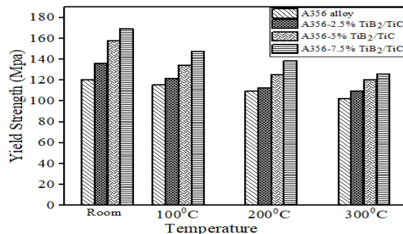
Fig. 8. Influence of temperature YS composites.
