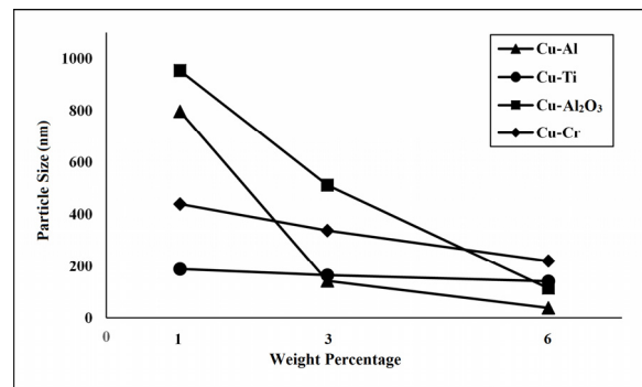
Fig. 5. Particle Size Distribution of the synthesized samples.
