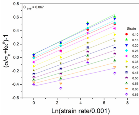
Fig. 4. Plot of \frac{\sigma}{\sigma_o + K\varepsilon^n} - 1 vs. \ln \dot{\varepsilon} at reference condition.
