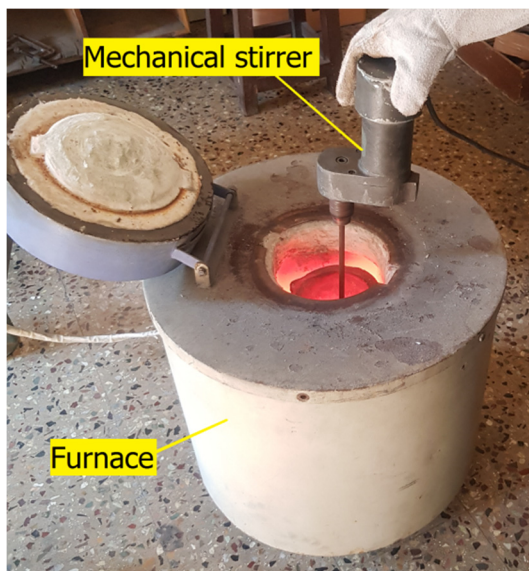
Fig. 1. Stir casting setup and Die used for preparing MMC
