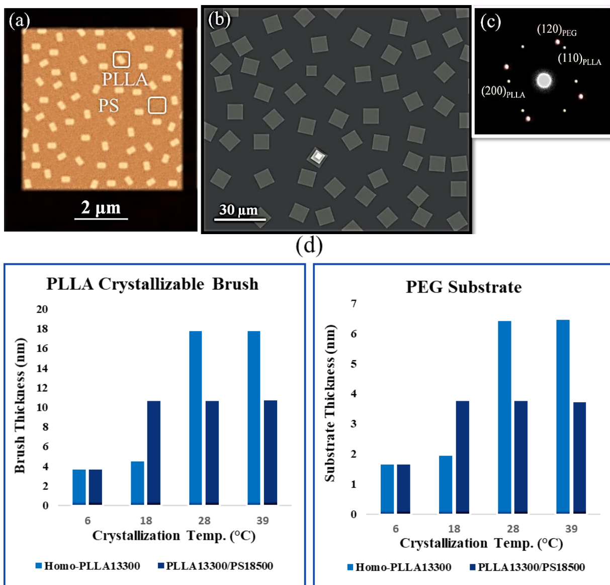
Fig. 4. AFM height image (a) and the corresponding SAED pattern (c) of PEG 5000 - b -PS 18500 /PEG 5000 - b -PLLA 13300 single crystals grown at T c = 18°C, in which the PLLA brushes are crystalline; STEM image of PEG 5000 - b -PS 18500 /PEG 5000 - b -PLLA 13300 single crystals grown at T c = 39°C (b); the thickness trends of PLLA brushes and PEG substrate via altering the crystallization temperature in PEG 5000 - b -PLLA 13300 and PEG 5000 - b -PS 18500 /PEG 5000 - b -PLLA 13300 single crystals (d).
