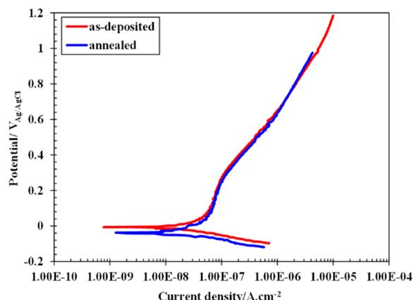
Fig. 7. PDP curves of (a) as-deposited and (b) annealed specimens in Ringer’s solution.
