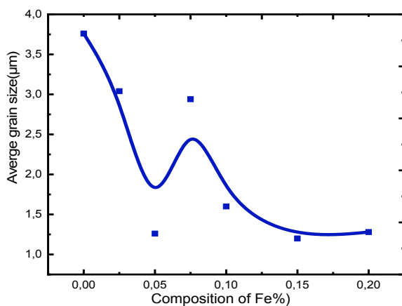
Fig. 5. Variation of grain size of PFZT ceramics sintered at 1100^{\circ}C for 4 h.
