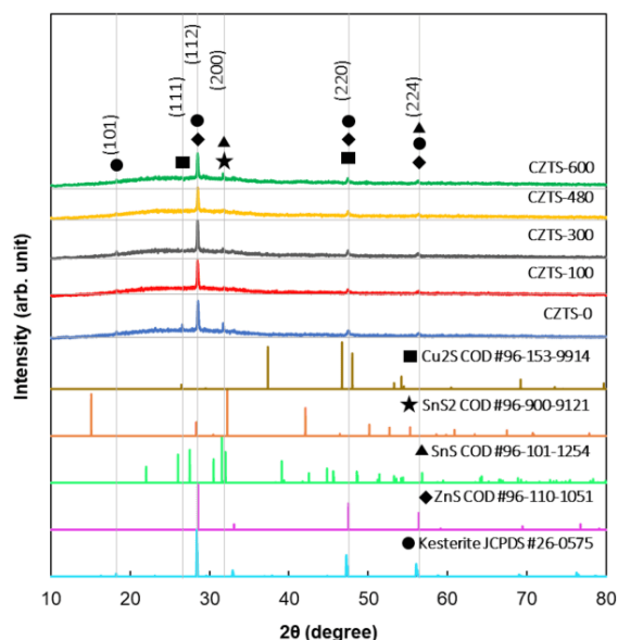
Fig. 6. XRD diffraction patterns show the formation of ZnS, Cu_2S , SnS, and SnS_2 as secondary phases
