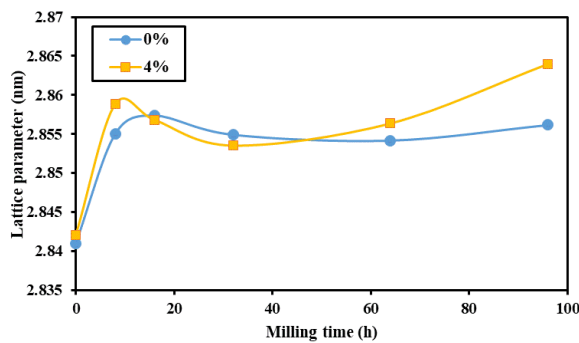
Fig. 8. Variations of lattice parameter versus different milling times for \text{Fe}_{80}\text{Ni}_{20} and (\text{Fe}_{80}\text{Ni}_{20})_{96}\text{Cr}_4
