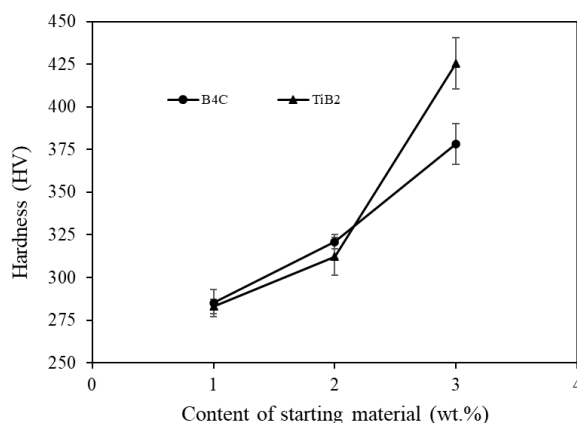
Fig. 8. Variation of hardness with the additive content.
