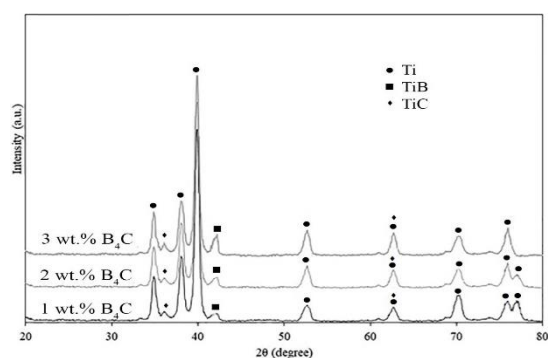
Fig. 4. XRD patterns of the samples synthesized using B_4C .
