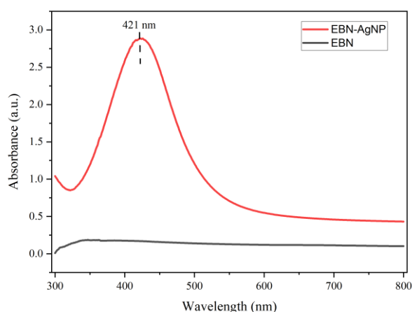
Fig. 2. UV-visible spectra of sample synthesised by the reaction of AgNO_3 (800 \mu L, 0.05 M) reacted with EBN extracted at a concentration of 6 wt. %.
