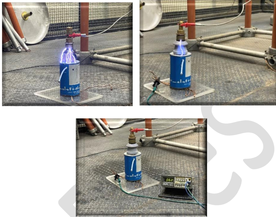
Fig. 11. The setup for the breakdown voltage test (a) the uncoated and (b) the coated (S33) samples, together with the setup for the leakage current test (c)
