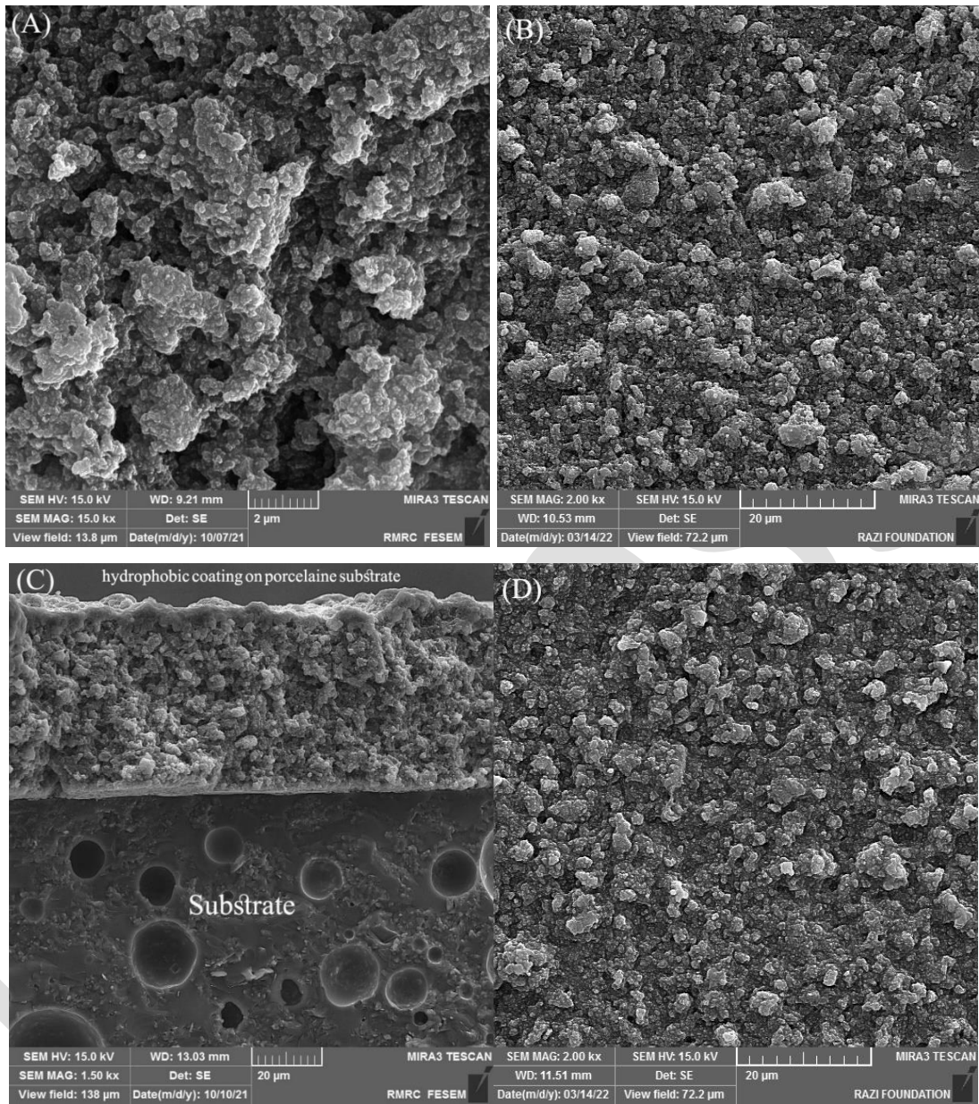
Fig. 7. FESEM images of the coatings, (A) S31, (B) S33, (D) S35, and (C) the cross section of S33 on the glazed porcelain insulator
