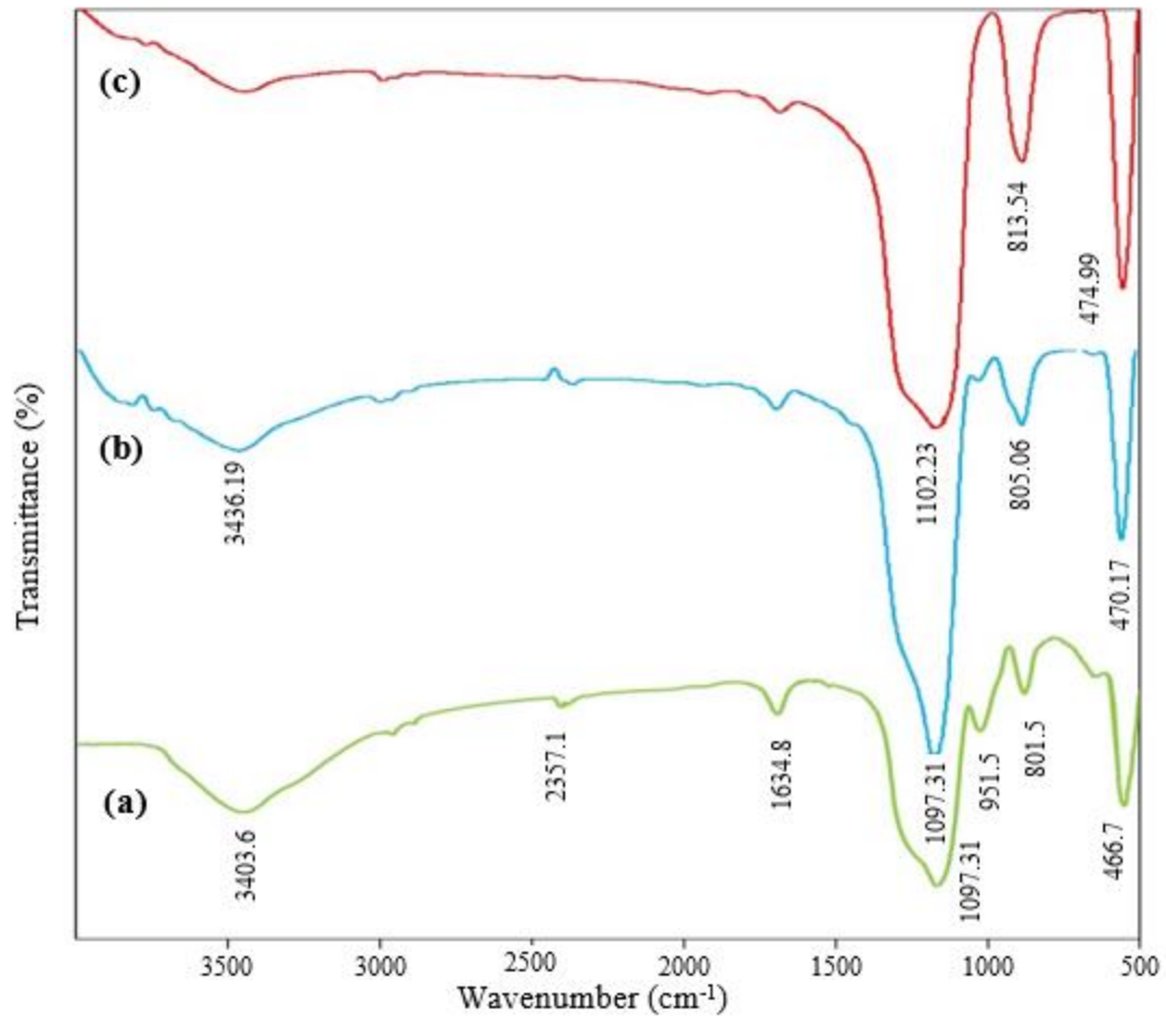
Fig. 2. The FTIR patterns of a) silica nanoparticles, b) silica nanoparticles hydrophobized with ODTS, and c) silica nanoparticles hydrophobized with HMDS
