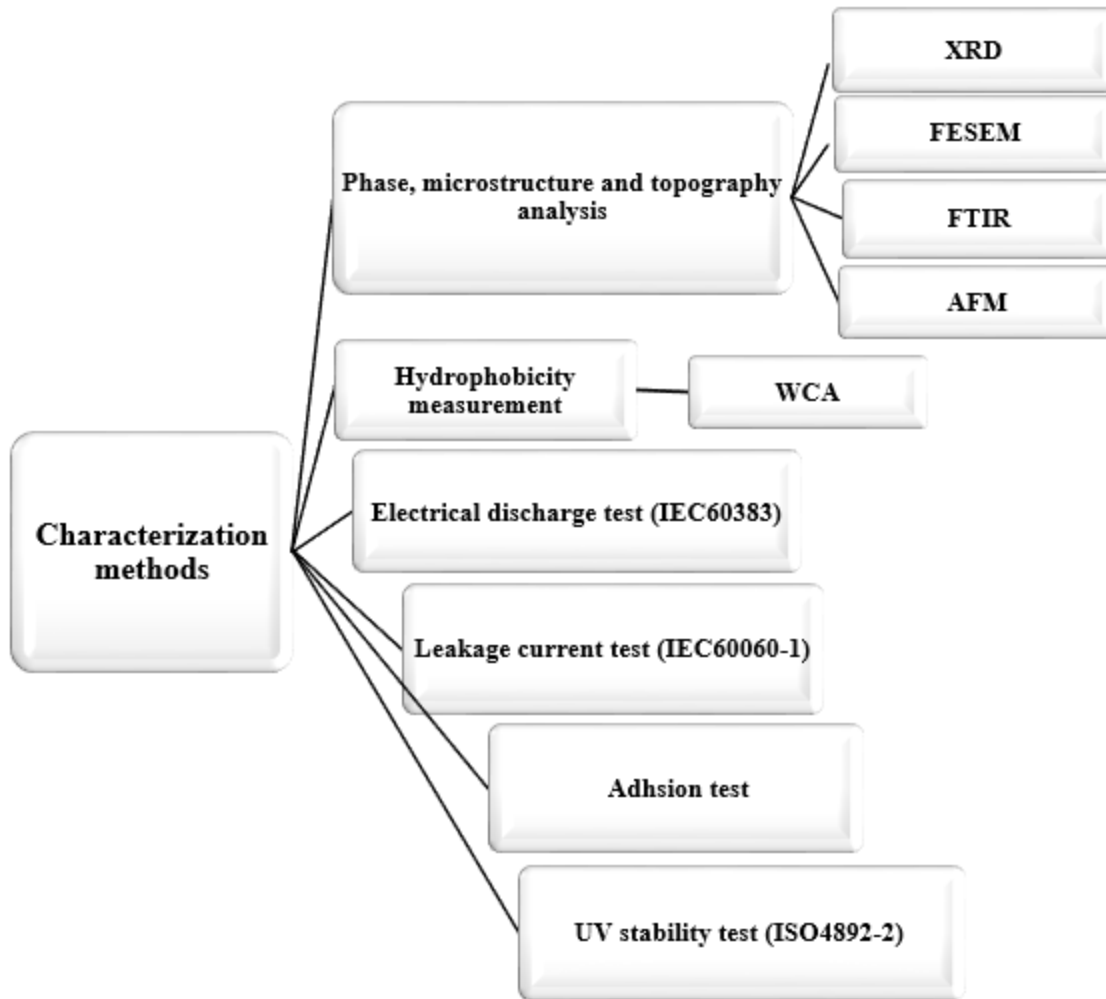
Fig. 1. Characterization methods to characterize the coated samples
