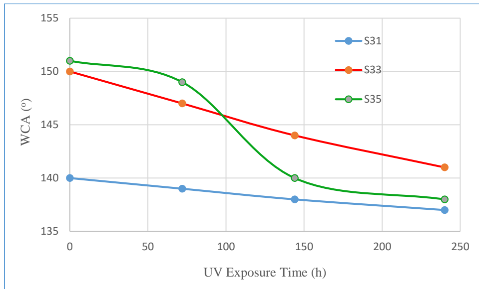
Fig. 10. The Effect of UV irradiation on WCA
