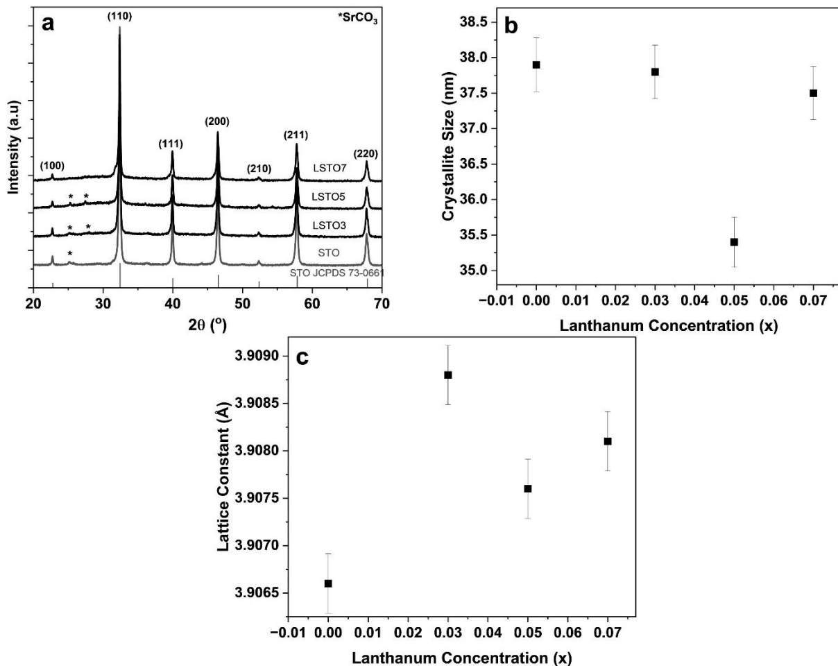
Fig. 1. a) XRD patterns, b) crystallite size, and c) lattice constant of STO and LSTO samples
