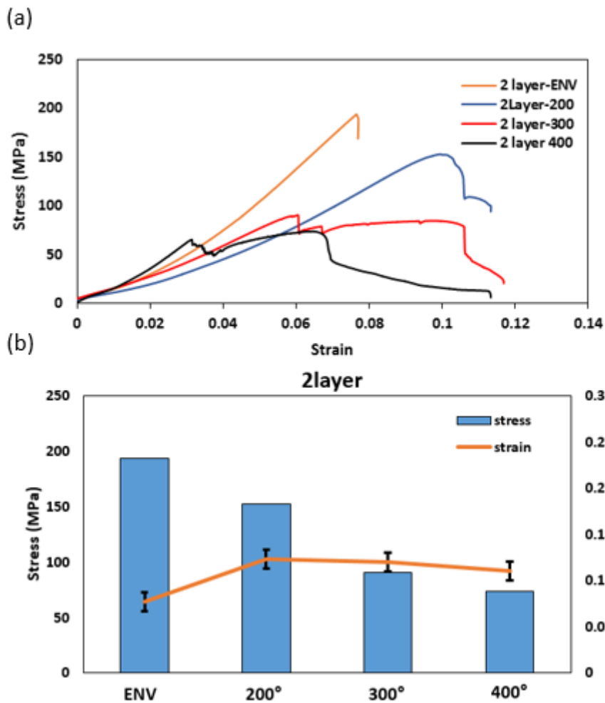
Fig. 9. (a) Engineering Stress-Strain curves of two-layer sheets in environment temperatures, 200°C, 300°C and 400°C, (b) Investigating the effect of different annealing temperature conditions on strain and stress
