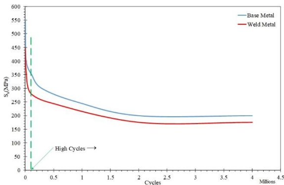
Fig. 7. Stress amplitude–fatigue life results of the base metal of Haynes 25 alloy (blue) and the weld zone of the alloy (red)
