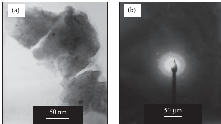
Fig. 3. TEM image of Mg_2Ni-5 \text{ wt\% } TiO_2 composite: (a) light-field image (b) electron diffraction pattern.
