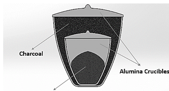
Mixture of Celestite and Graphite Fig. 2. Experimental setup for placing celestite and graphite mixture in a charcoal bed
