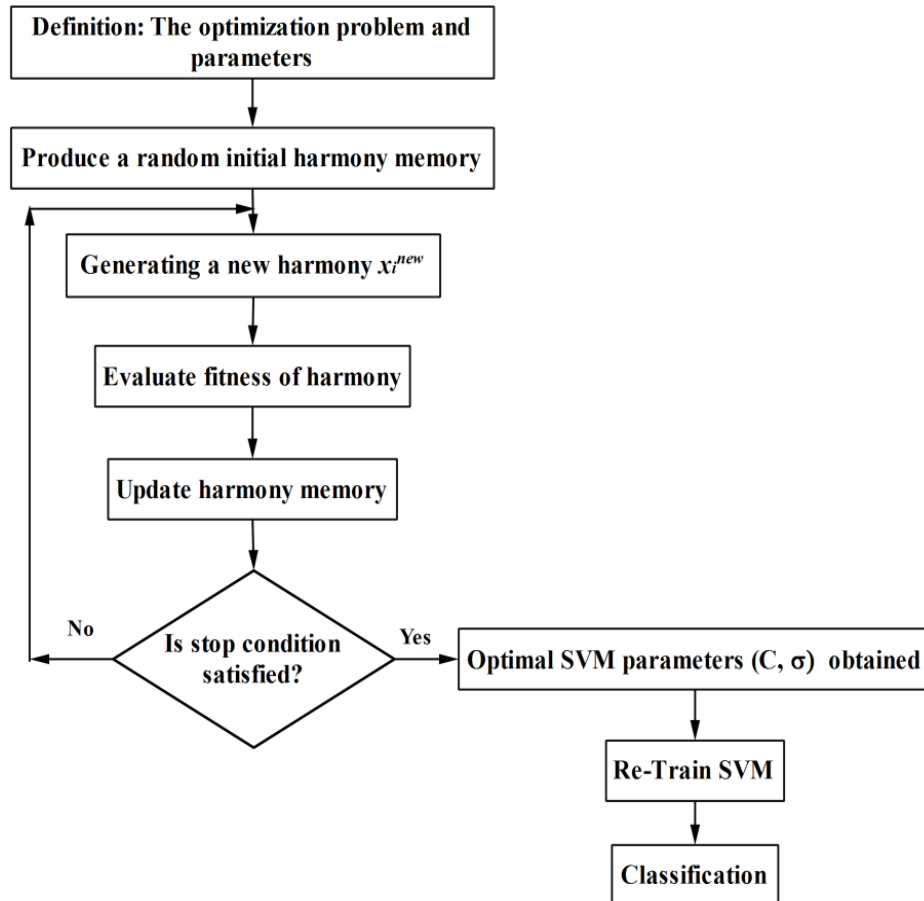
Figure 3. The process of optimizing the SVM parameters with the HS
