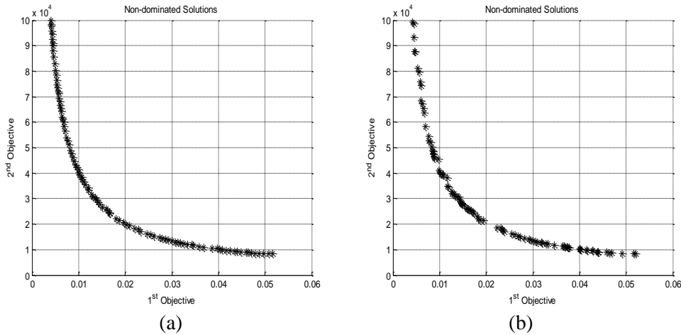
Figure 13. Resulted Pareto front by (a) NSGA-II and (b) MOFPSO for the truss sizing at TP5
