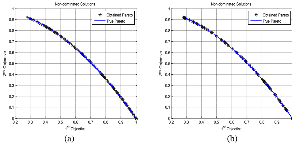
Figure 11. Resulted Pareto front by (a) NSGA-II and (b) MOFPSO for TP3
