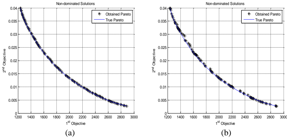
Figure 12. Resulted Pareto front by (a) NSGA-II and (b) MOFPSO for 4bar truss design (TP4)
