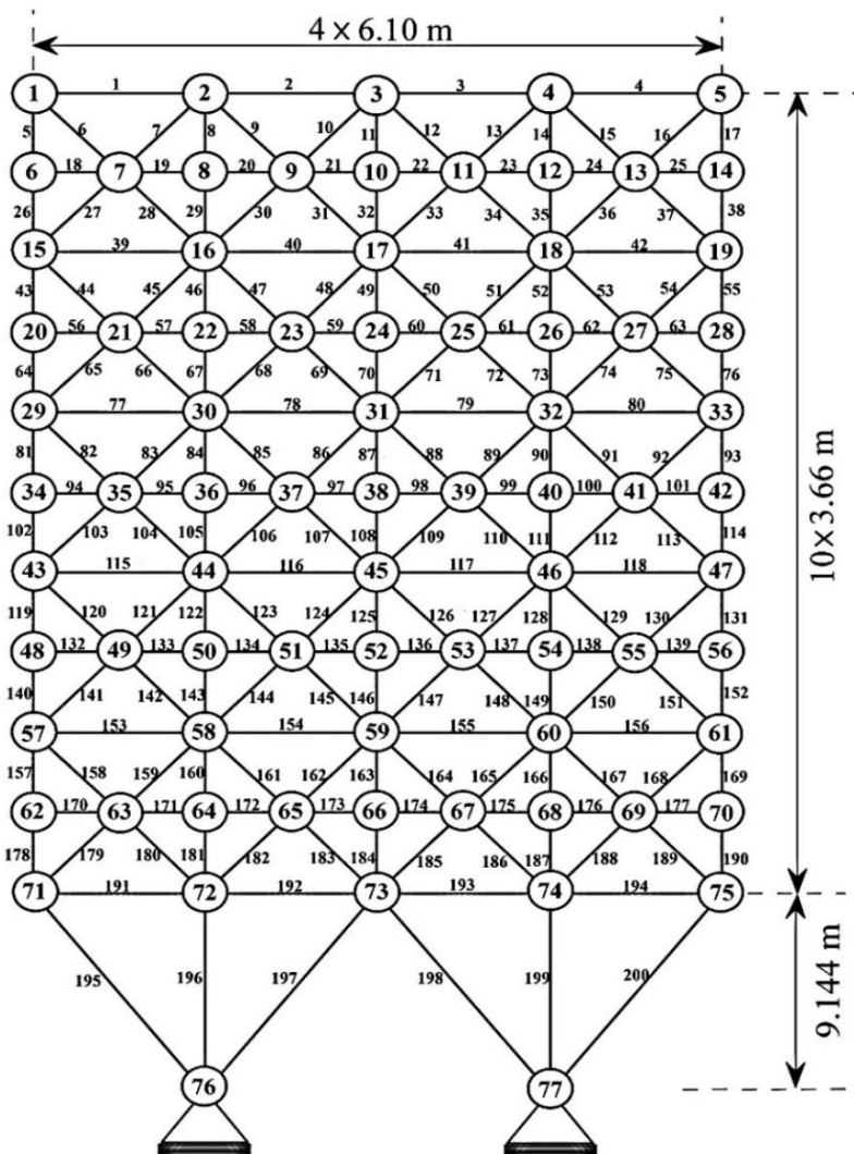
Figure 3. Schematic of the 200-bar planar truss [21]
