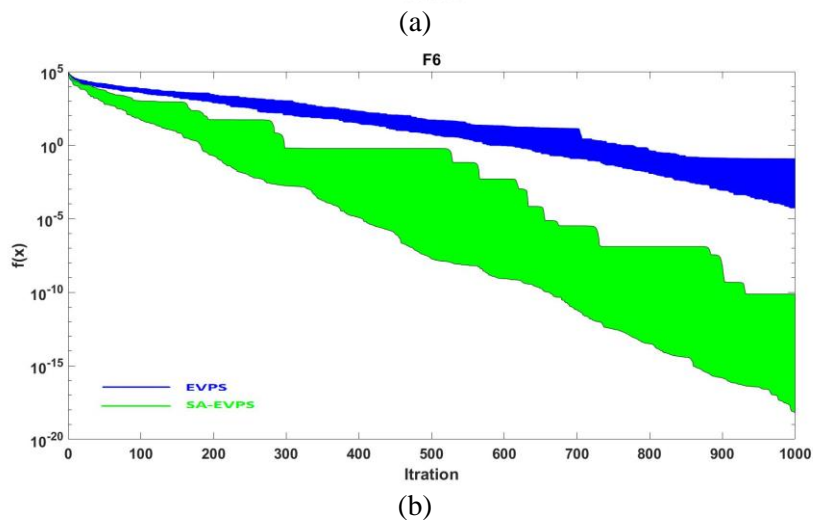
Figure 9. Convergence curves for 30 independent runs of the F_6 function are shown in Table 3. (a) graph in linear form, (b) graph in solid form
