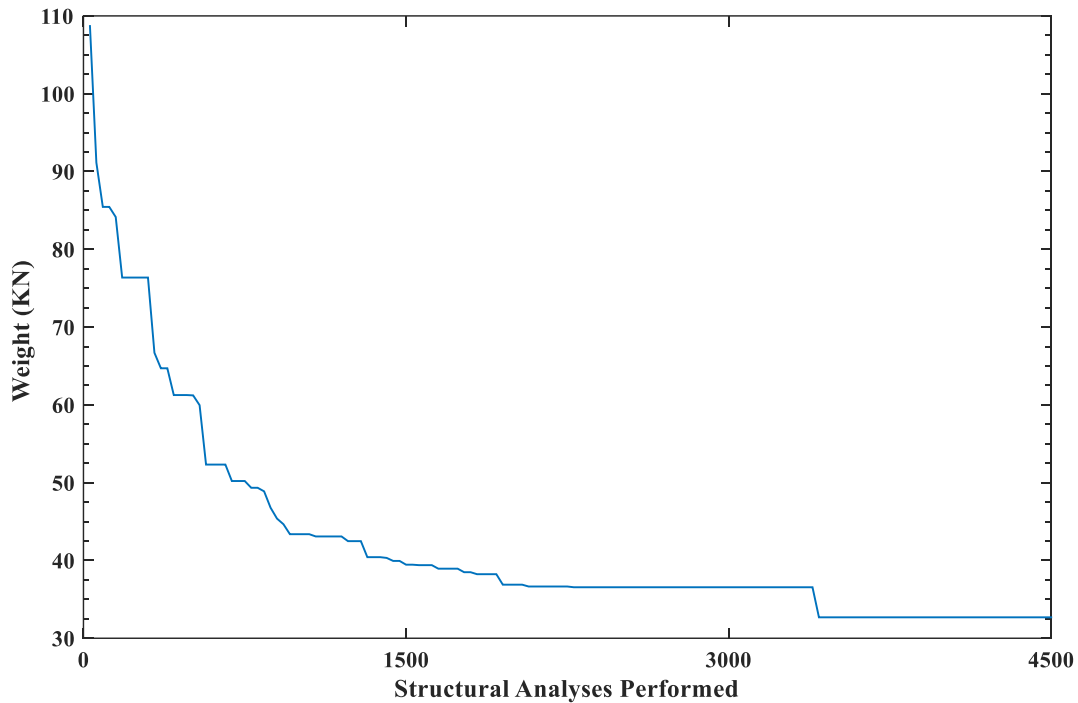
Figure 10. Convergence histories related to the best results of 1×8 frame
