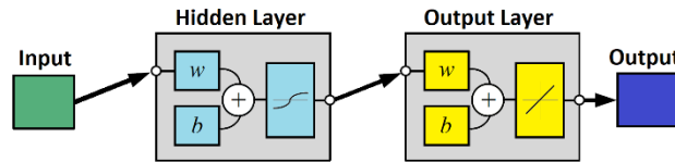
Figure 2. FFBP neural network model
