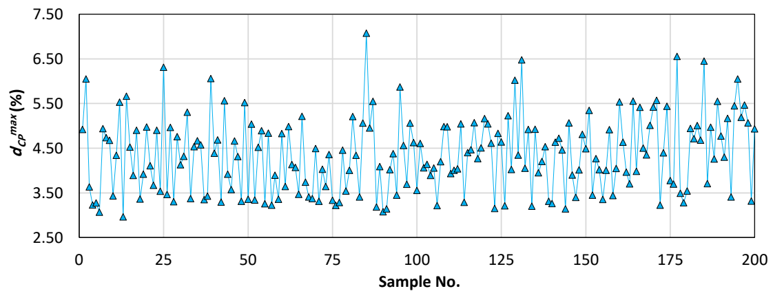
Figure 9: Maximum inter-story drift ratios at the CP level for the 6-story frame
