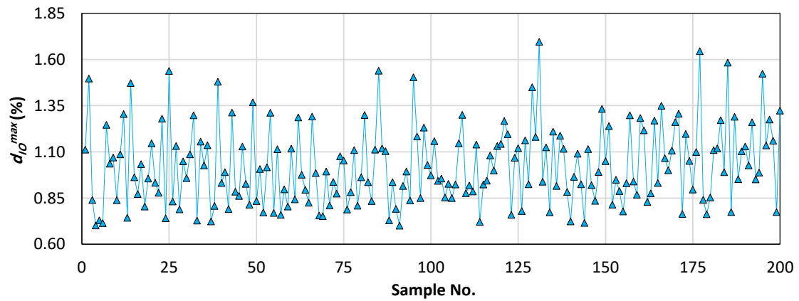
Figure 7: Maximum inter-story drift ratios at the IO level for the 6-story frame
